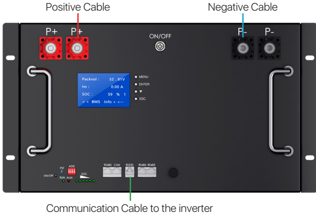
Positive Cable Communication Cable Negative Cable
