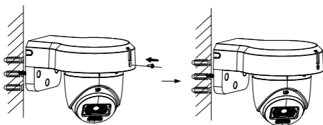
Figure 2-34 Lock Cover to Body
