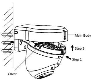
Figure 2-68 Secure Cover to Body
