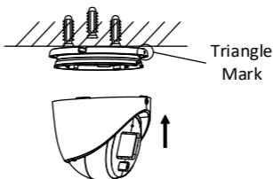
Figure 2-38 Install Camera Back
