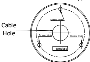
Figure 2-1 Drill Template
