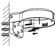
Figure 2-31 Secure Main Body to Wall
