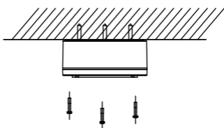
Figure 2-43 Combine Junction Box Cover and Body
