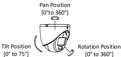
Figure 2-39 3-Axis Adjustment
