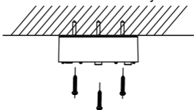
Figure 2-42 Secure Junction Box Body
