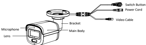
Figure 1-1 Overview of Type I Camera
