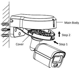
Figure 2-12 Secure Cover to Body
