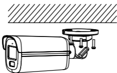
Figure 2-15 Secure Camera to Ceiling
