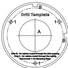
Figure 2-22 Drill Template for Junction Box
