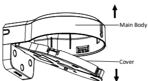
Figure 2-29 Take Apart Wall Mount
