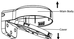
Figure 2-64 Take Apart Wall Mount
