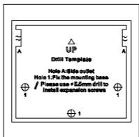
Figure 2-9 Drill Template for Wall Mount
