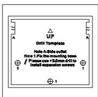
Figure 2-65 Drill Template for Wall Mount
