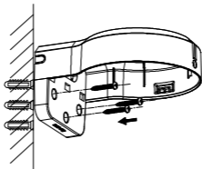
Figure 2-66 Secure Main Body to Wall
