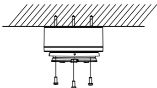
Figure 2-44 Fix Base
