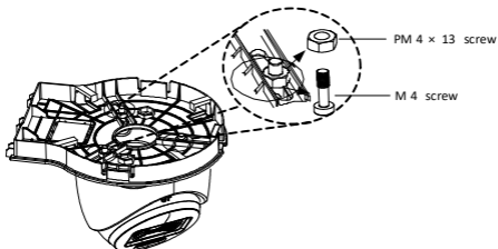
Figure 2-32 Secure Camera to Wall Mount Cover
