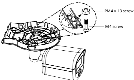
Figure 2-11 Secure Camera to Wall Mount Cover
