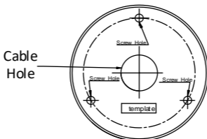
Figure 2-14 Drill Template
