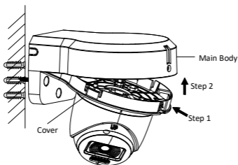
Figure 2-33 Secure Cover to Body
