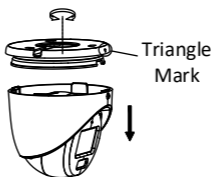
Figure 2-35 Disassemble Camera
