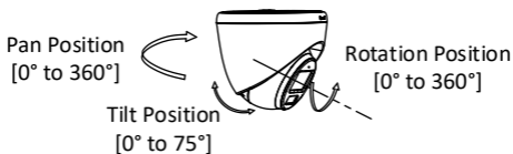
Figure 2-54 3-Axis Adjustment
