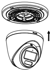
Figure 2-57 Fit Camera
