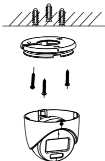
Figure 2-37 Secure Base to Ceiling
