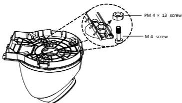
Figure 2-67 Secure Camera to Wall Mount Cover
