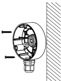
Figure 2-6 Secure Junction Box on Wall
