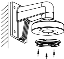
Figure 2-48 Fix the Base onto the Wall Mount
