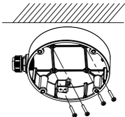
Figure 2-59 Secure Junction Box Body
