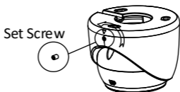
Figure 2-40 Loosen the Set Screw
