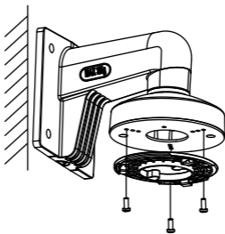
Figure 2-62 Fix Gang Box
