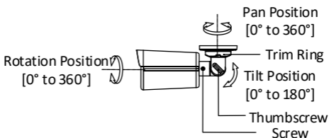
Figure 2-16 3-Axis Adjustment
