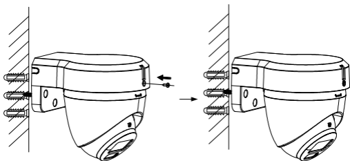
Figure 2-69 Lock cover to Body
