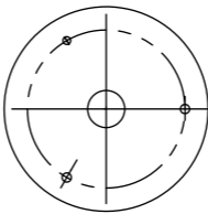
Figure 2-50 Drill Template
