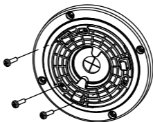
Figure 2-56 Install Gang Box to Junction Box Cover
