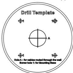
Figure 2-55 Drill Template
