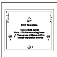
Figure 2-30 Drill Template for Wall Mount
