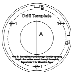
Figure 2-41 Drill Template for Junction Box
