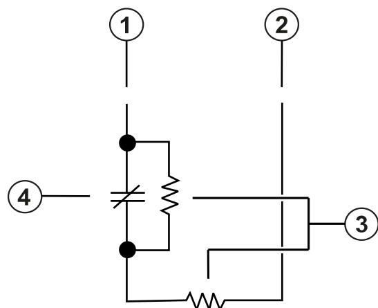
Figure 5: DEOL wiring
