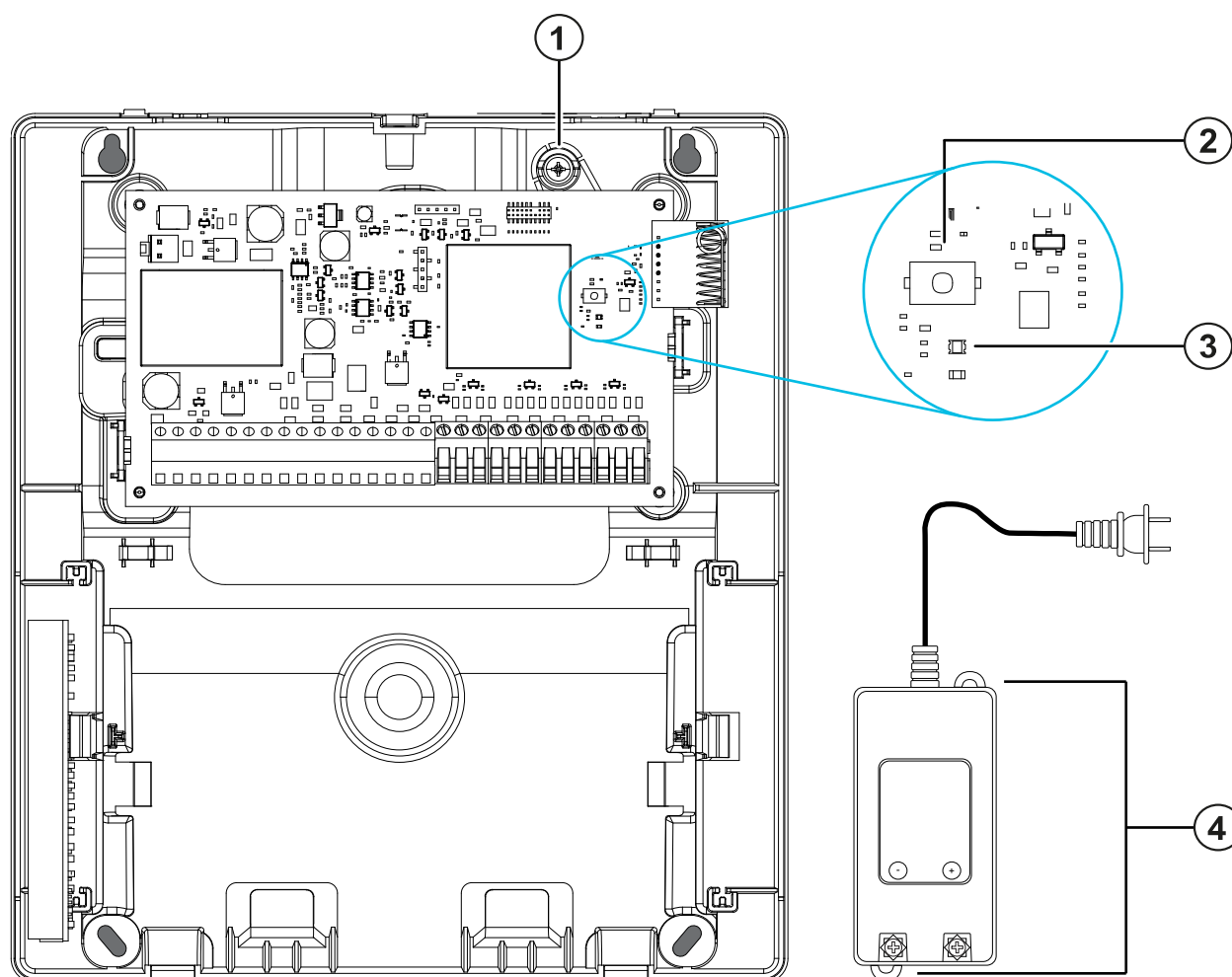
Figure 2: Mounting locations
