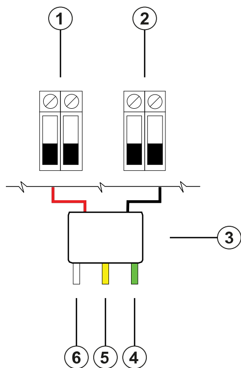
Figure 7: Relay output wiring
