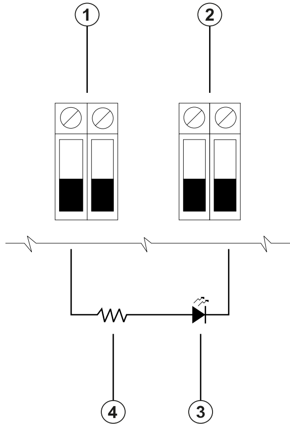
Figure 6: LED indicator wiring
