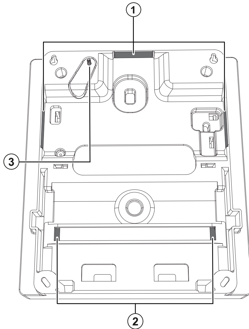
Figure 1: Breakaway tabs and battery strap slots
