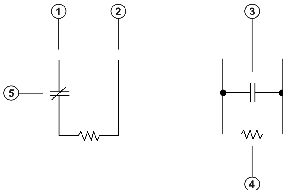
Figure 4: SEOL wiring
